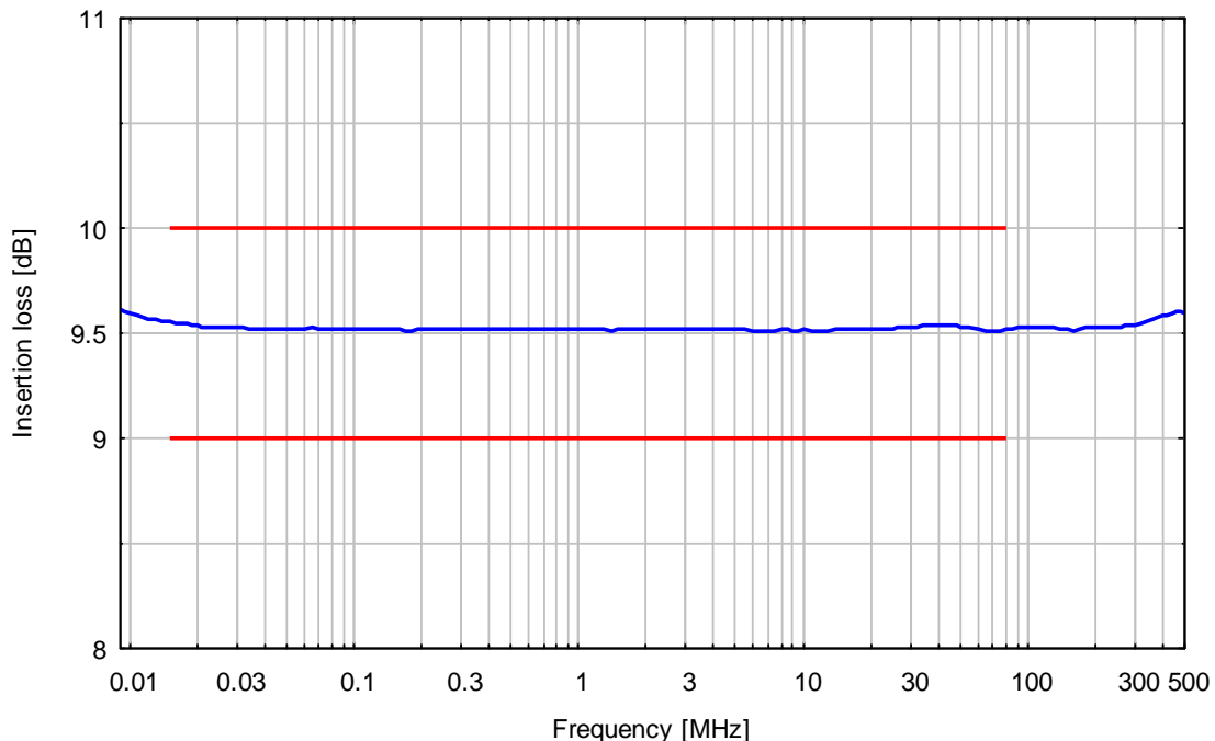
Insertion Loss acc. to EN 61000-4-6
